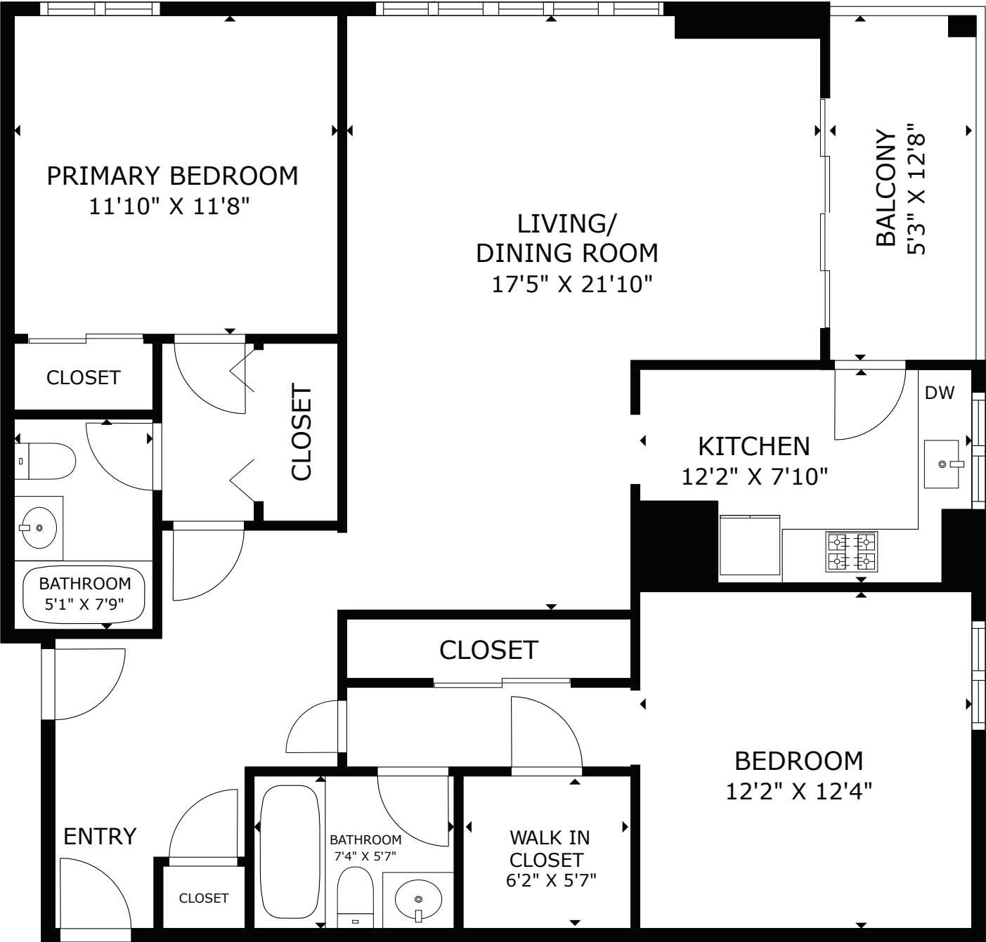
FLOOR PLAN
