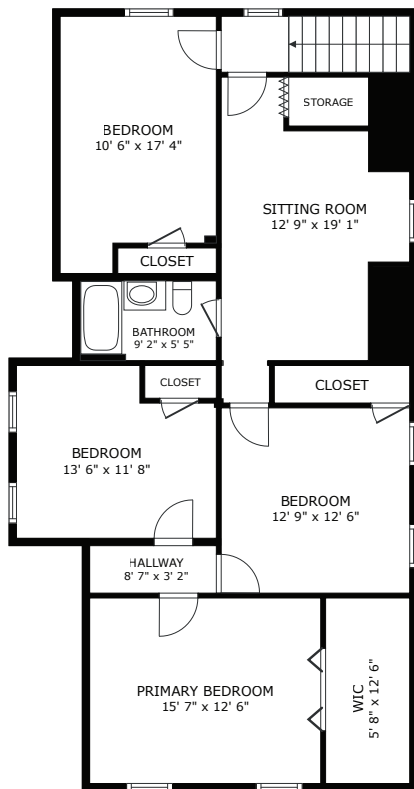
UPPER LEVEL - UNIT 2
