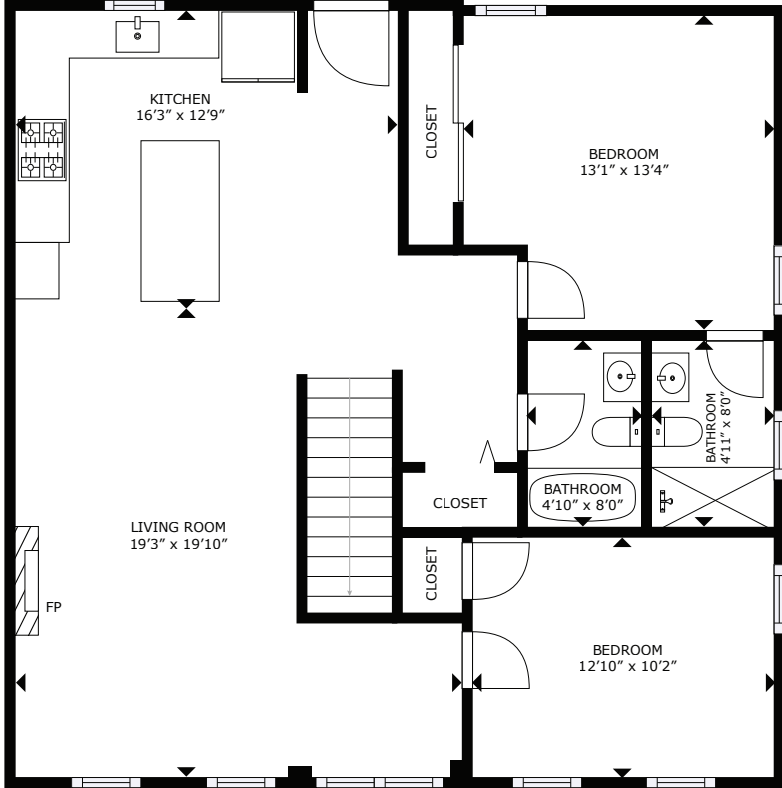
FLOOR 2
