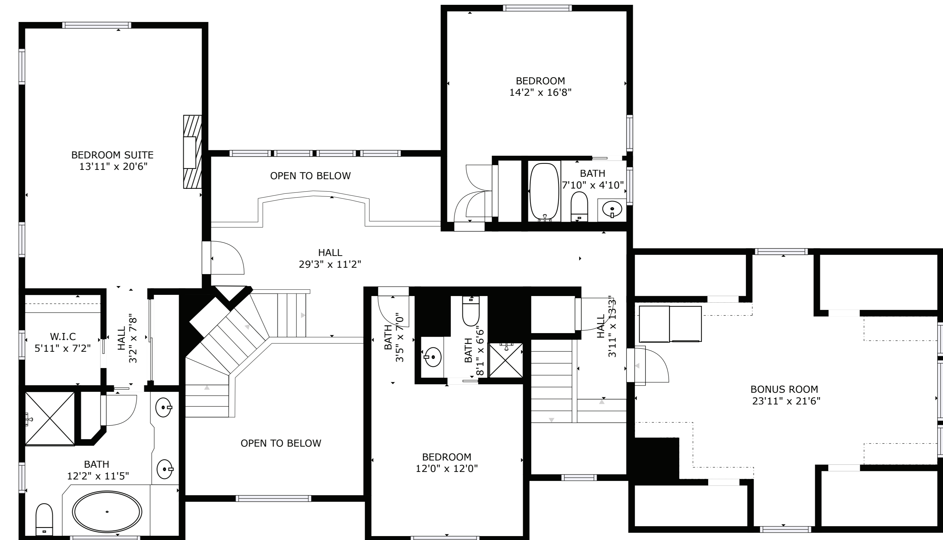
FLOOR 3
